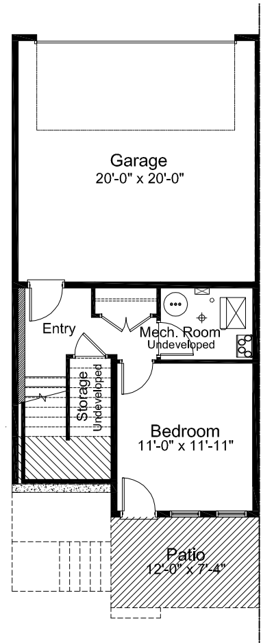
Lower Floor: 234 sq. ft.
