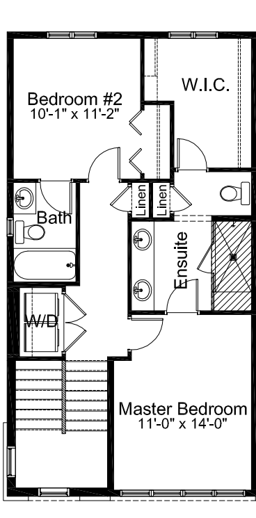
Upper Floor: 738 sq. ft
