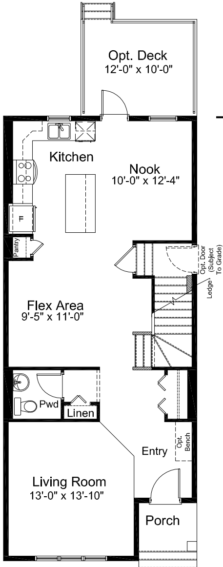
MAIN FLOOR: 884 SQ. FT.
