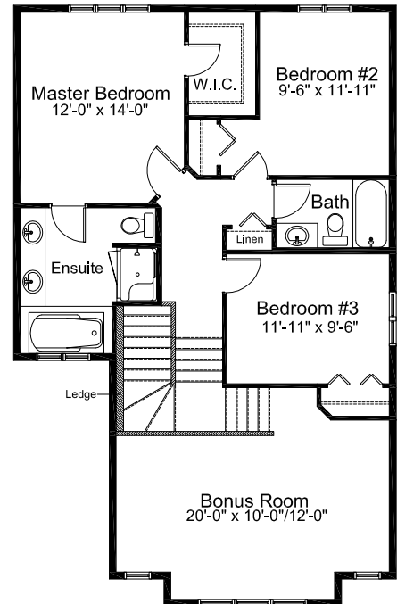
Upper Floor 1089 sq. ft.
